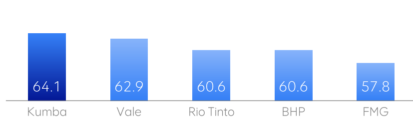
Fe qualities (%)
